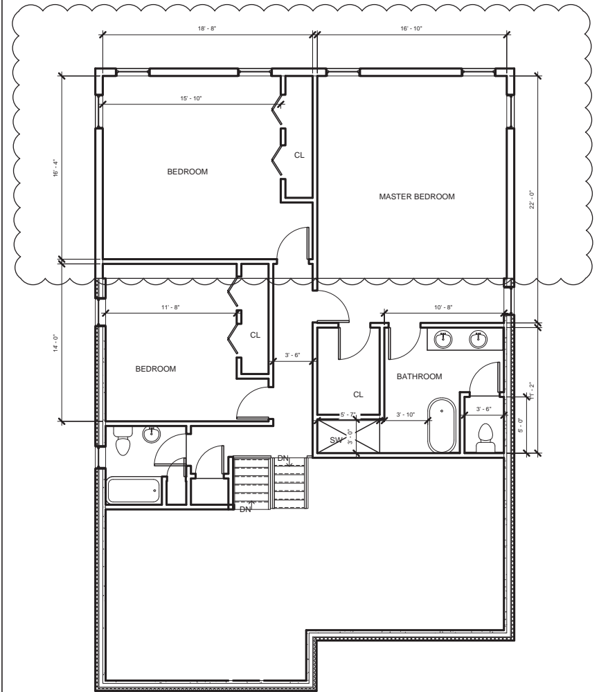
PROPOSED - 2ND FLOOR PLAN SCALE:
