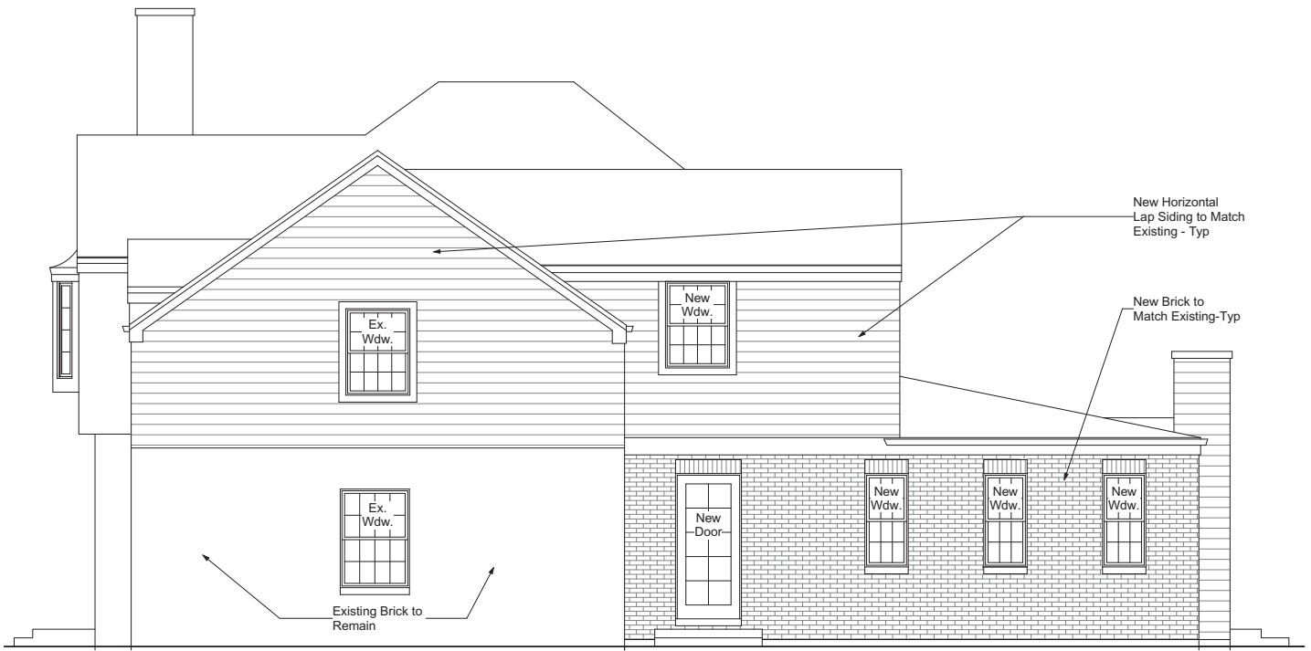
North Elevation 1/4" = 1'-0"
