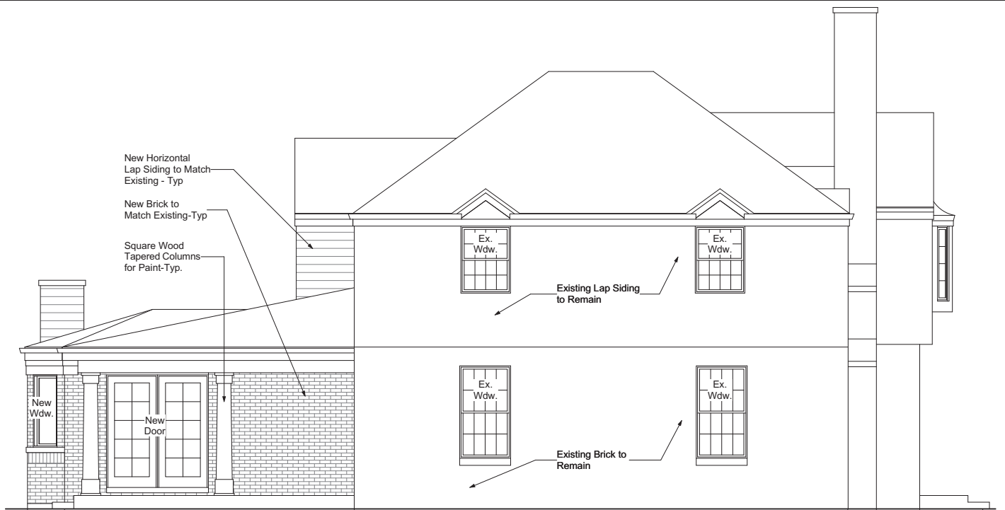
South Elevation 1/4" = 1'-0"
